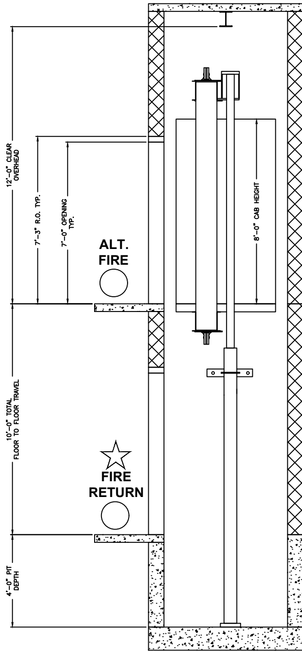
ELEVATION VIEW HOISTWAY
