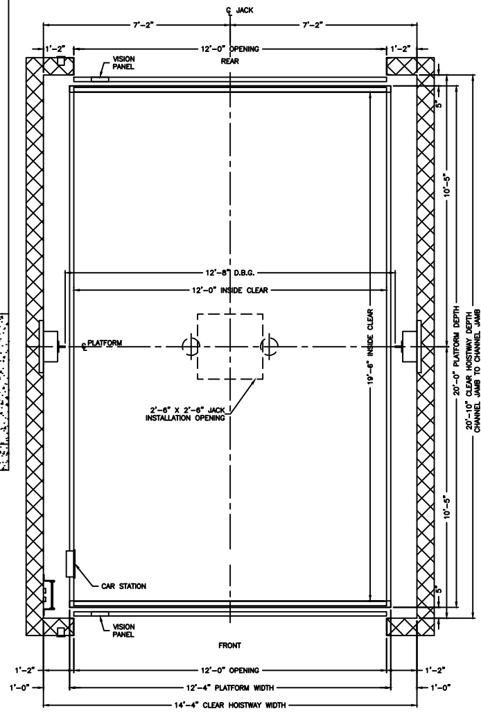
PLAN VIEW HOISTWAY
