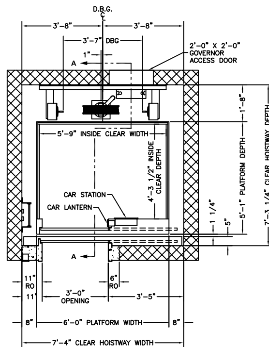
PLAN VIEW HOISTWAY
