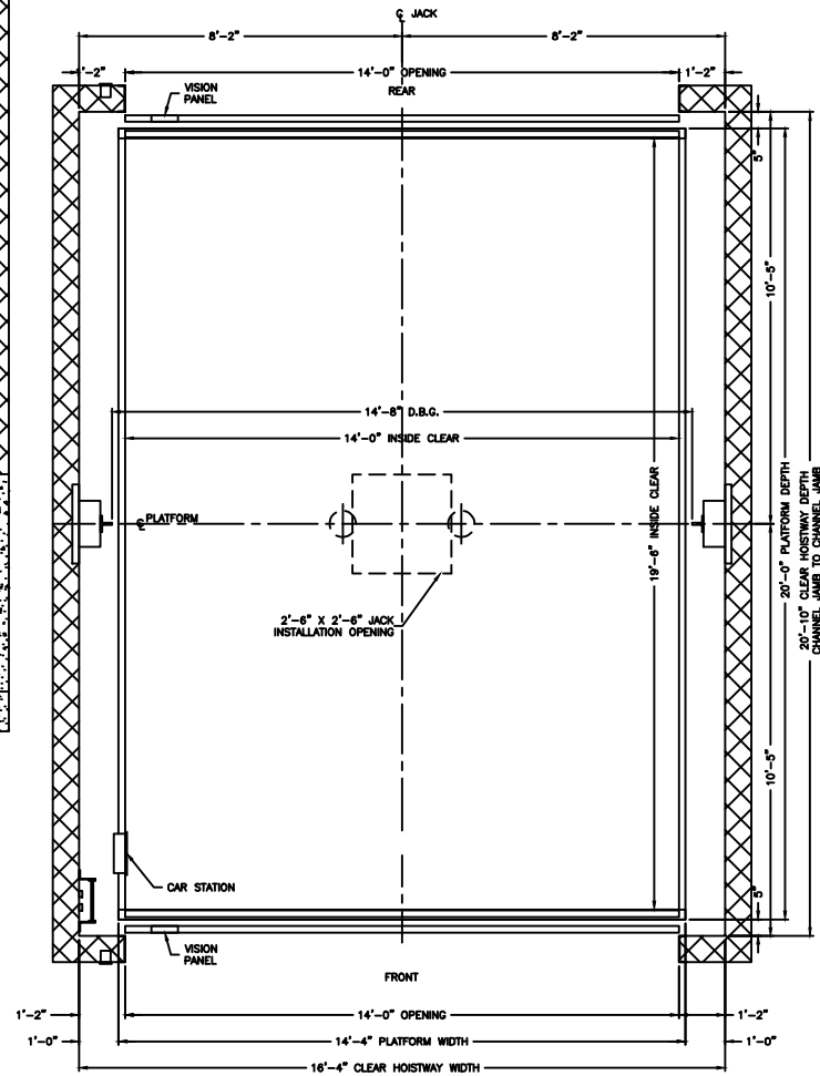
PLAN VIEW HOISTWAY
