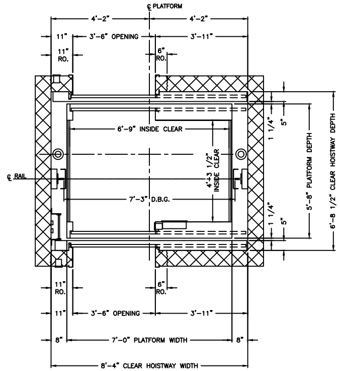
PLAN VIEW HOISTWAY
