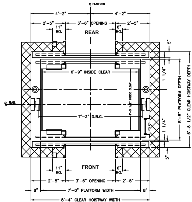
PLAN VIEW HOISTWAY
