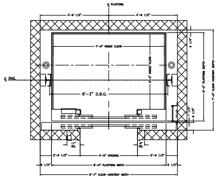
PLAN VIEW HOISTWAY
