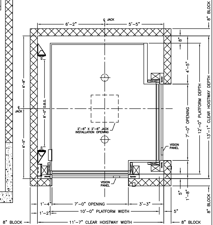
PLAN VIEW HOISTWAY
