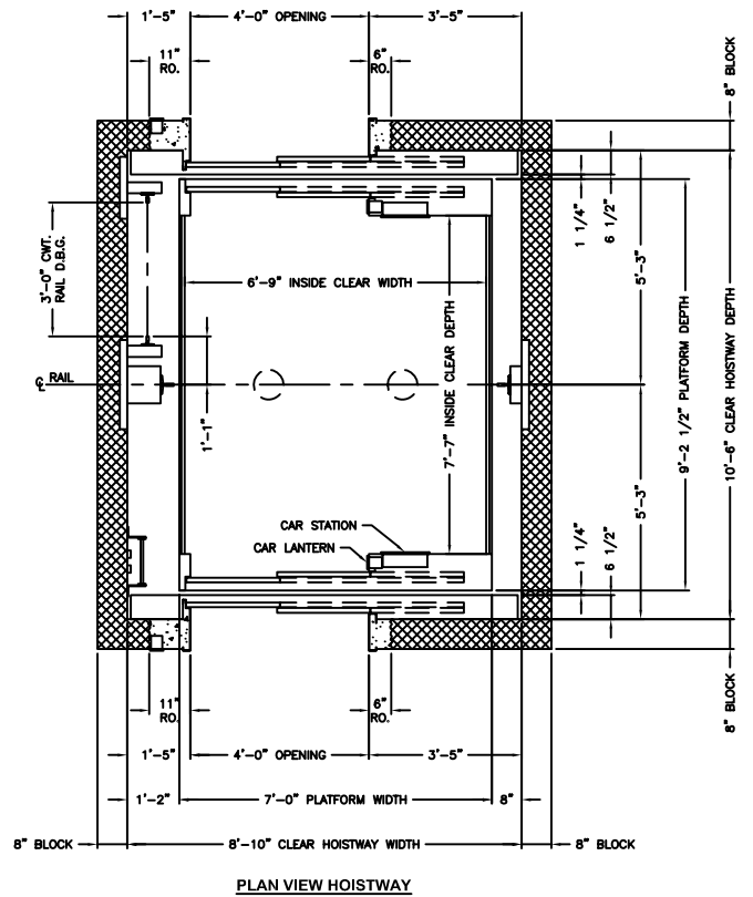
PLAN VIEW HOISTWAY
