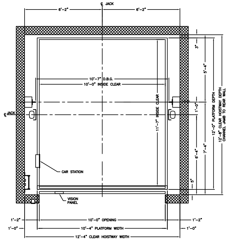
PLAN VIEW HOISTWAY
