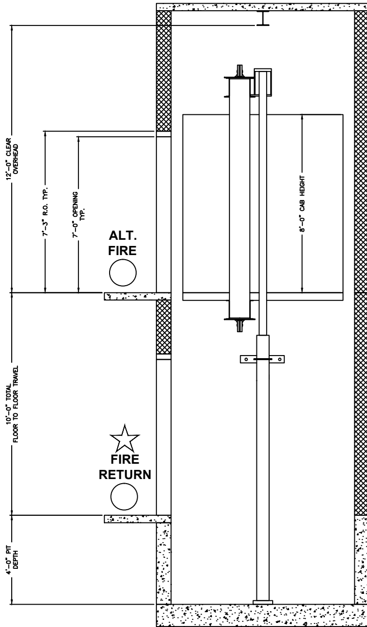
ELEVATION VIEW HOISTWAY
