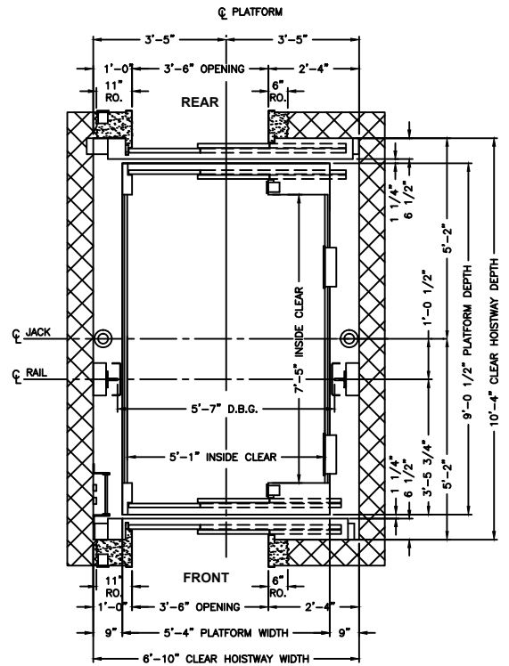
PLAN VIEW HOISTWAY
