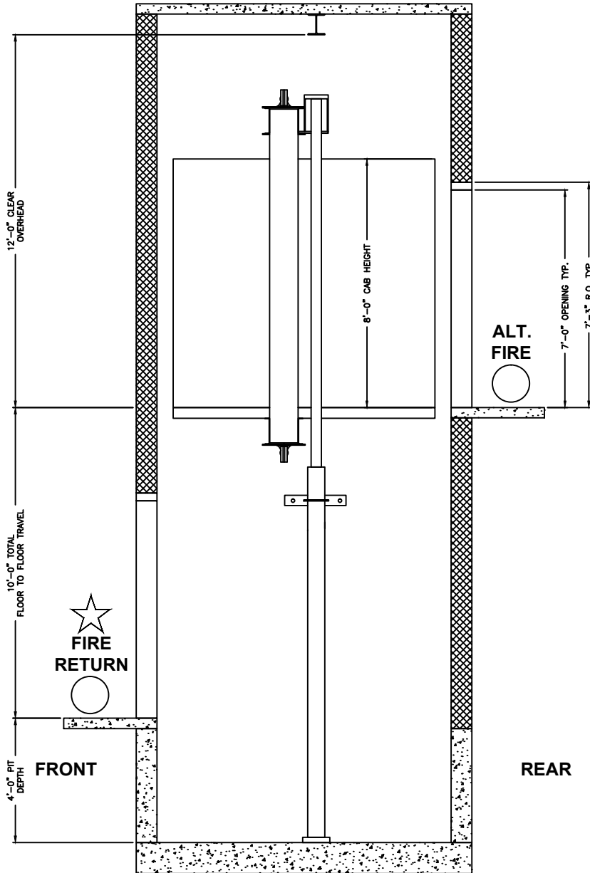
ELEVATION VIEW HOISTWAY
