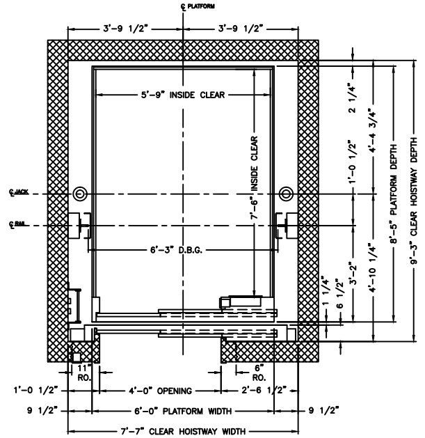
PLAN VIEW HOISTWAY
