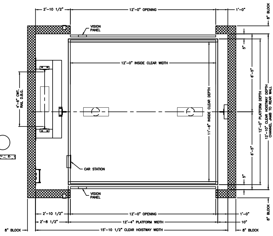
PLAN VIEW HOISTWAY
