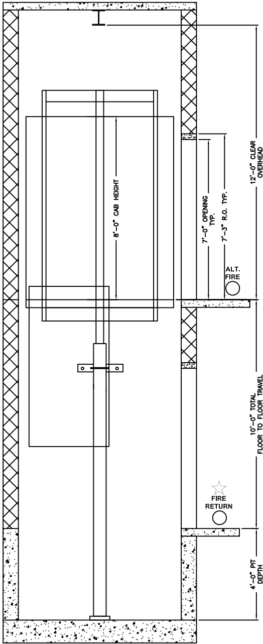
ELEVATION VIEW HOISTWAY
