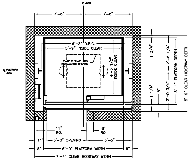
SIDE OPENING PLANVIEW
