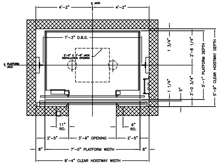
CENTER OPENING PLANVIEW
