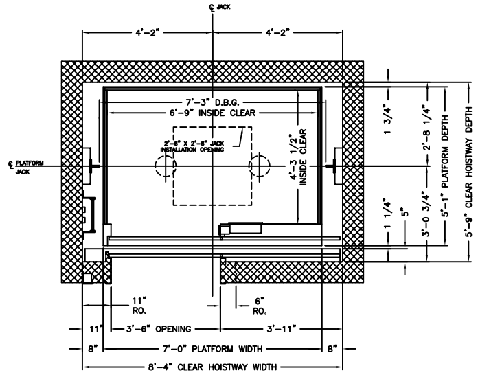
SIDE OPENING PLANVIEW
