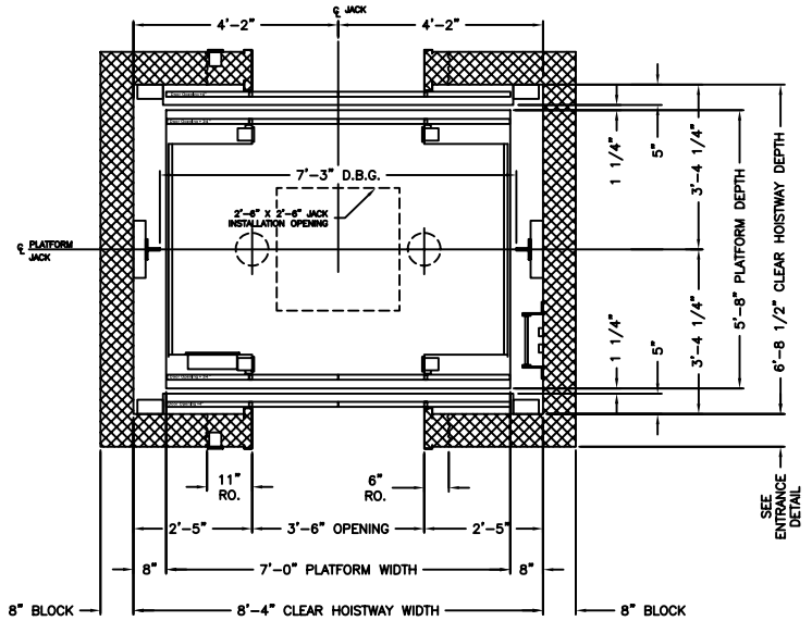
CENTER OPENING PLANVIEW
