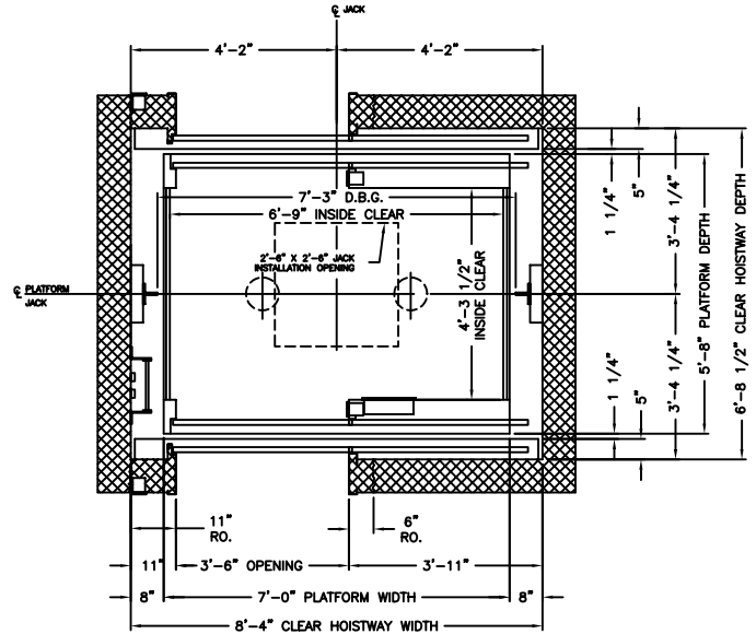
SIDE OPENING PLANVIEW
